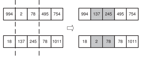
Figure 4. Crossover operation
